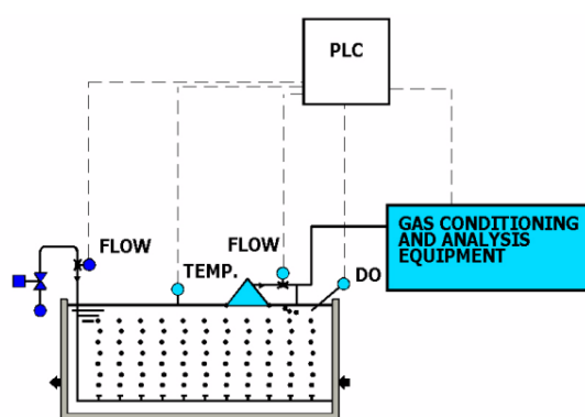
ALPHAMETER ® - Functional diagram
