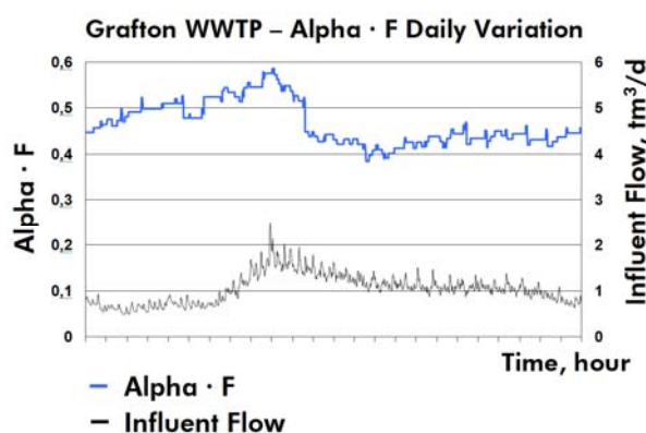
ALPHAMETER ® - Real plant data: Alpha·F daily variation
